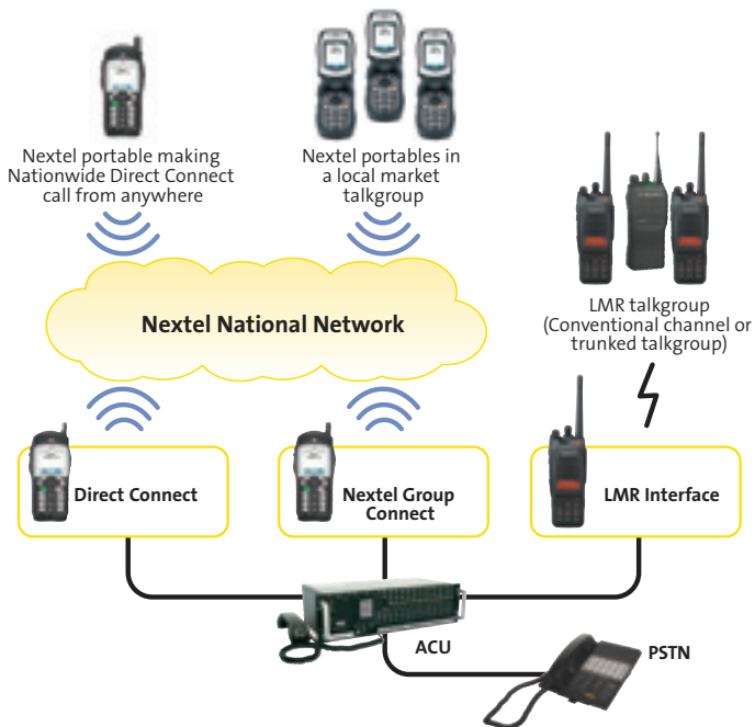
Figure 4. Combining Nextel Walkie-Talkie with Nextel Talkgroups with Land Mobile Radio talkgroups
